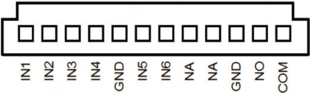
Figure 1-18 Alarm port
