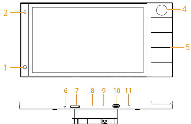
Figure 1-10 7-inch button central control screen with induction loop
