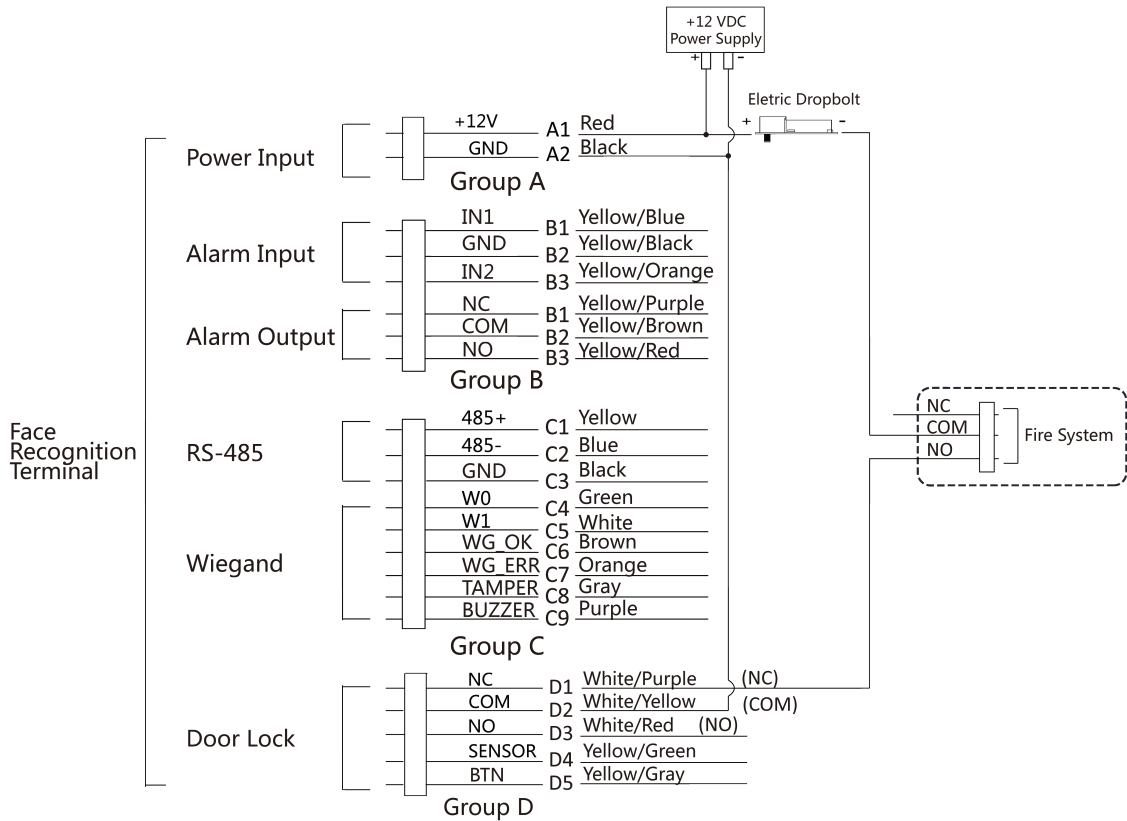
Figure 4-6 Wiring Device
