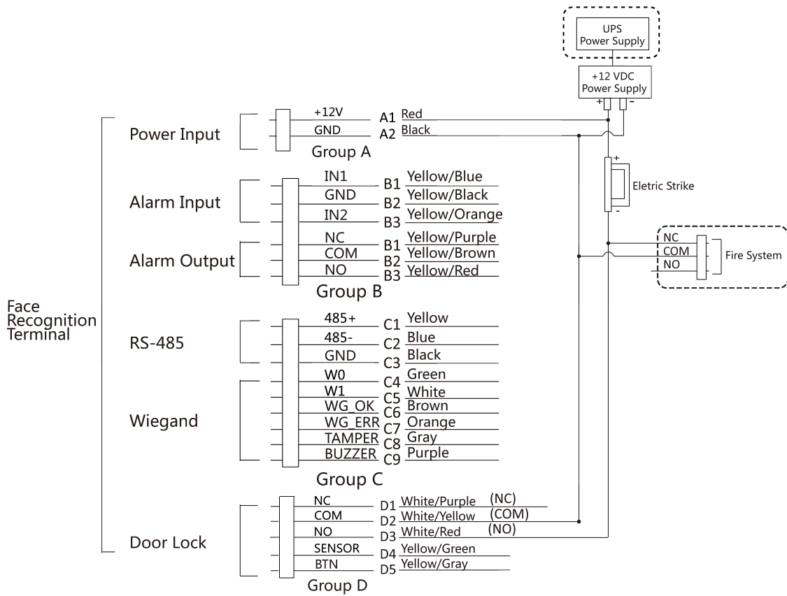
Figure 4-8 Device Wiring
