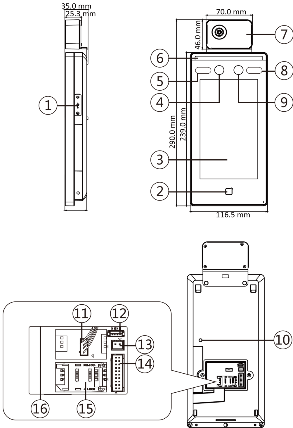
Figure 2-1 Face Recognition Terminal Diagram
