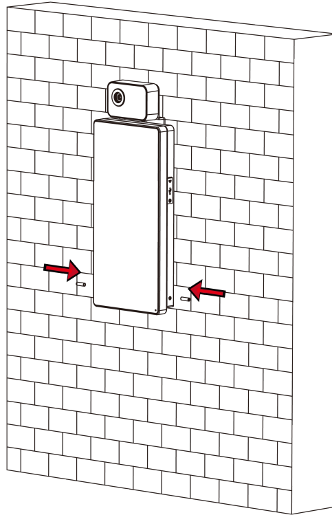
Figure 3-7 Secure Device
