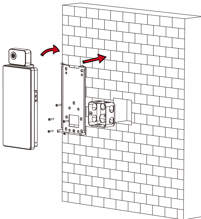
Figure 3-2 Install Device
