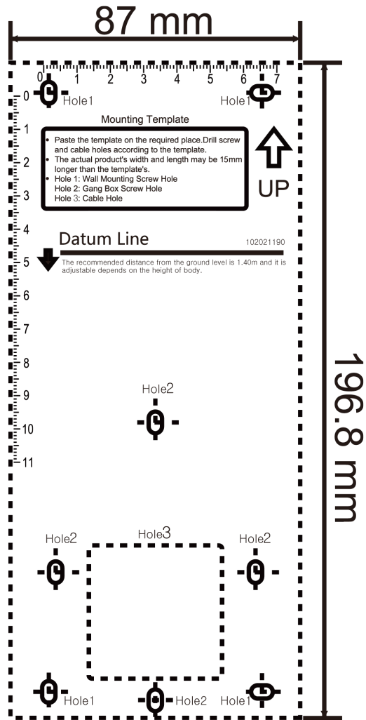
Figure 3-4 Mounting Template
