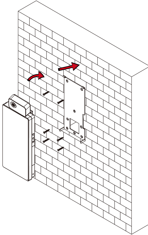
Figure 3-6 Install Device
