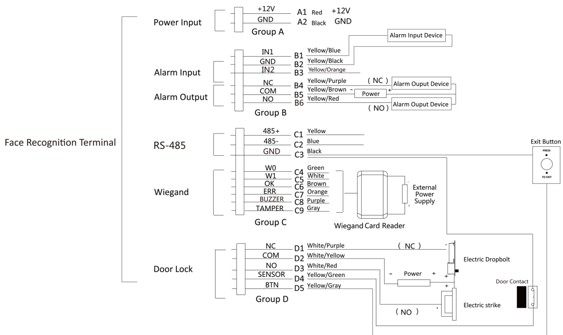
Figure 4-2 Device Wiring
