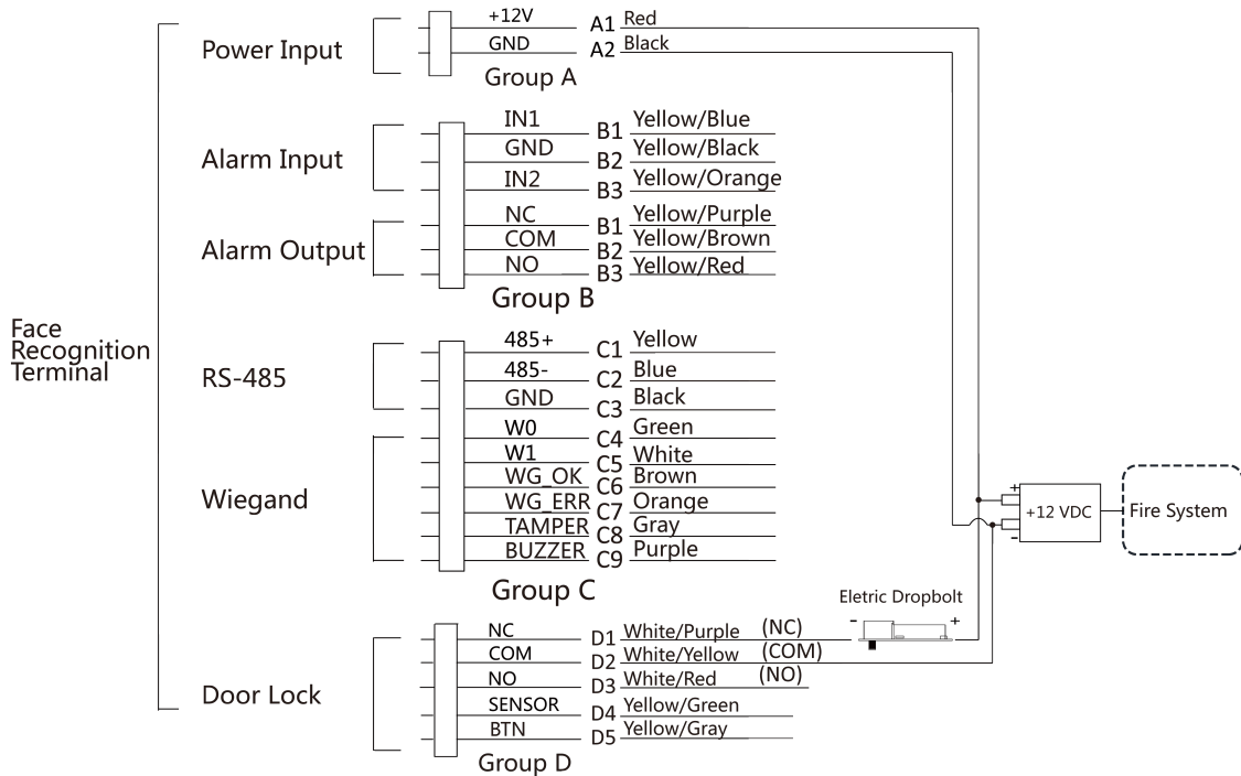
Figure 4-4 Wire Device
