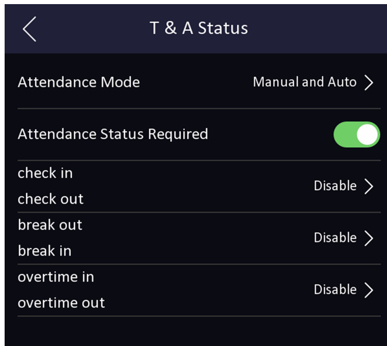
Figure 7-13 Manual and Auto Mode
