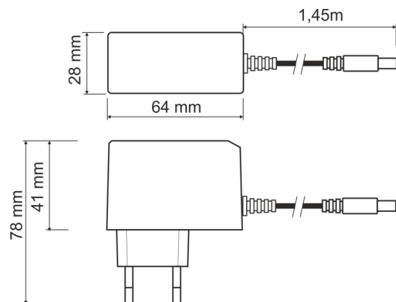
Fig.1. Dimensions of power supply.
